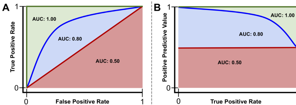
Figure 4. Example receiver operating characteristics and precision-recall curves. Red line : a model that performs no better than chance has an area under the curve (AUC) of the receiver operating characteristics curve (AUROC) of 0.50 or area under the precision-recall curve (AUPR) at the class ratio ( red shaded area ). Blue line : a model that performs better than chance, but not perfectly, will have an AUC between 0.50 and 1.00 ( blue + red shaded areas ). Green line : a model that performs perfectly has an AUC of 1.00 ( red + blue + green shaded areas ).
